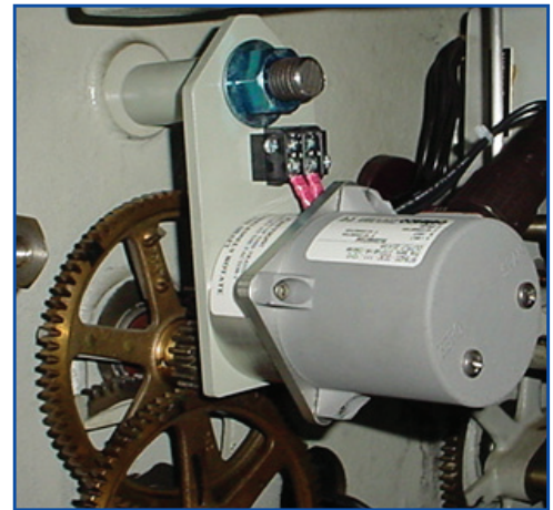
4-20mA Transmitter
