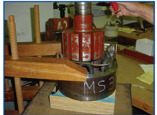
Pelton PMG Rotor entering fixture
