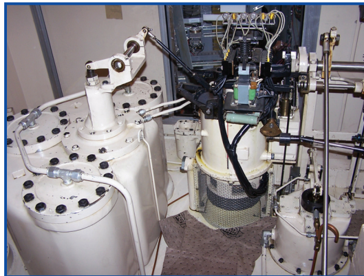
Pelton Mech Cab – Interior
